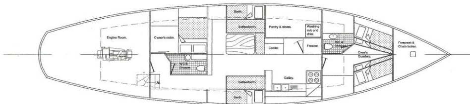
PLAN AT LOWER DECK.
