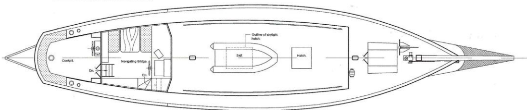
PLAN AT MAIN DECK.
