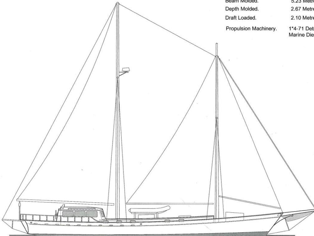
STARBOARD PROFILE.
